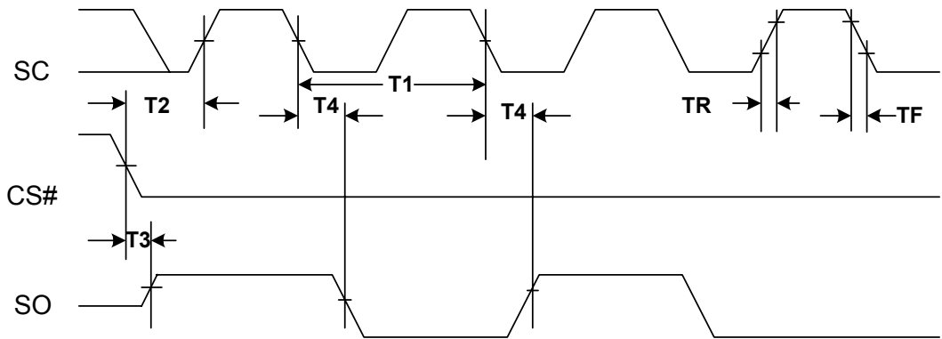
Data Output Timing Diagram
